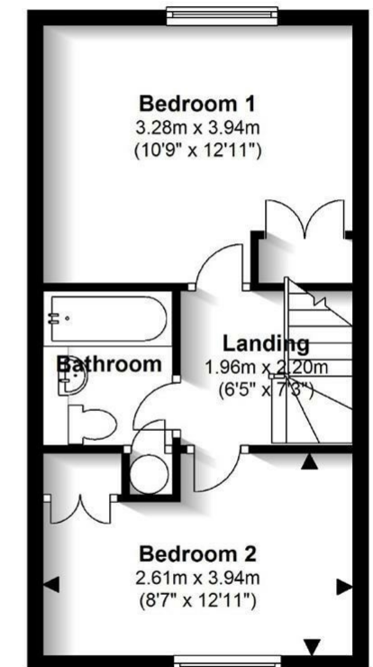
First Floor Approx. 31.7 sq. metres (340.7 sq. feet)
